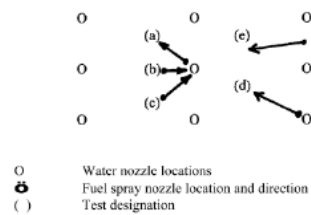
Figure 3.3.2 Fuel spray nozzle locations
