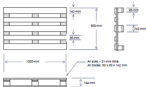
Figure 3.2.1 – Typical dimensions of the standard EUR pallet
