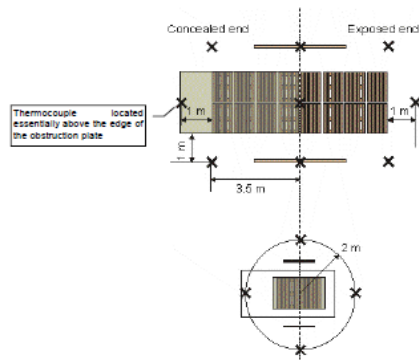
Figure 3.5.1 – Thermocouple locations in the two scenarios*
