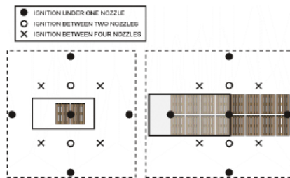
Figure 3.4.1 – Nozzle positioning in the two scenarios
