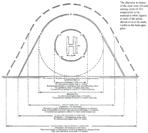
Figure 1: Landing area at the ship's side
