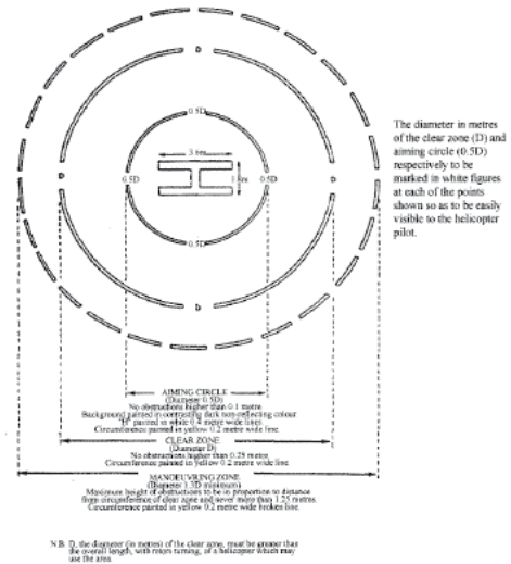
Figure 2: Landing area without unobstructed access from ship's side
