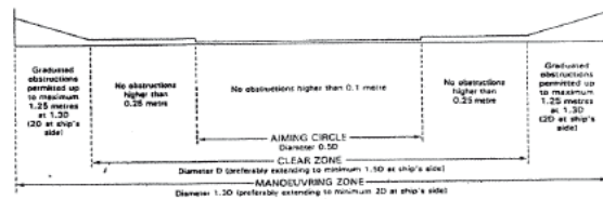
Figure 3: Landing area - permitted height of obstructions (elevation)
