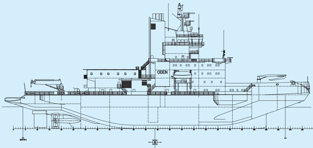
Building yard Götaverken AB, Arendal, Sweden, 1988.
